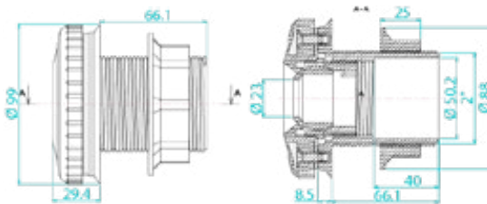
Code : 42231000 - With insert, jet and nut
